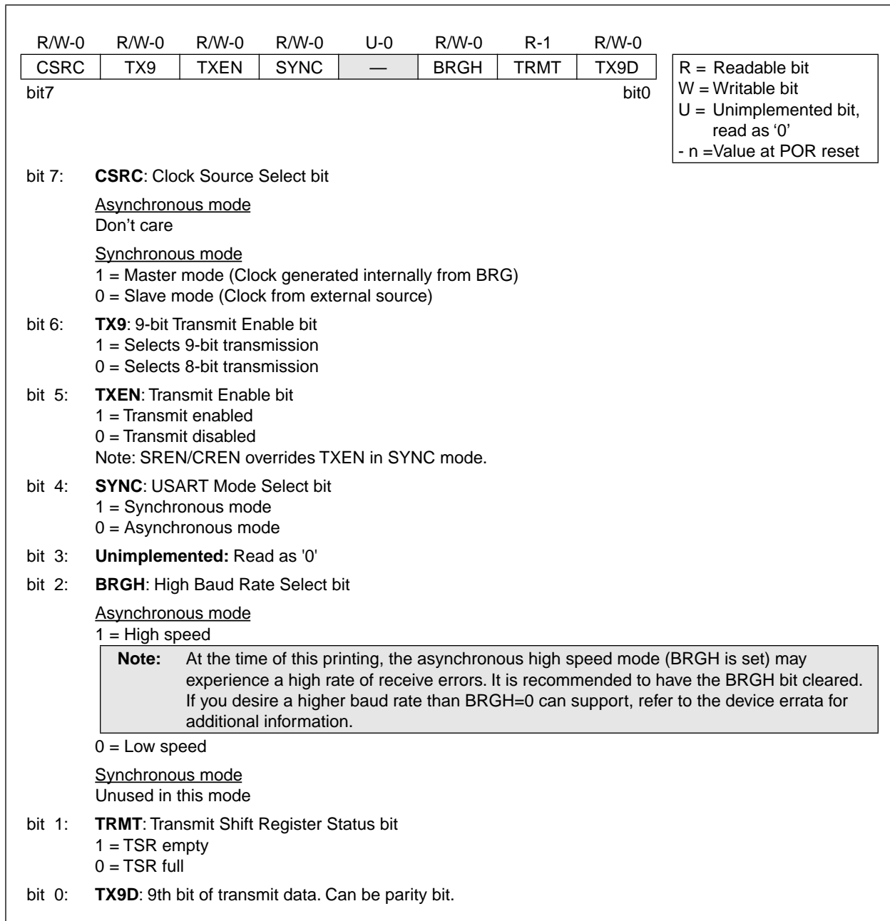
FIGURE 12-1: TXSTA: TRANSMIT STATUS AND CONTROL REGISTER (ADDRESS 98h)
