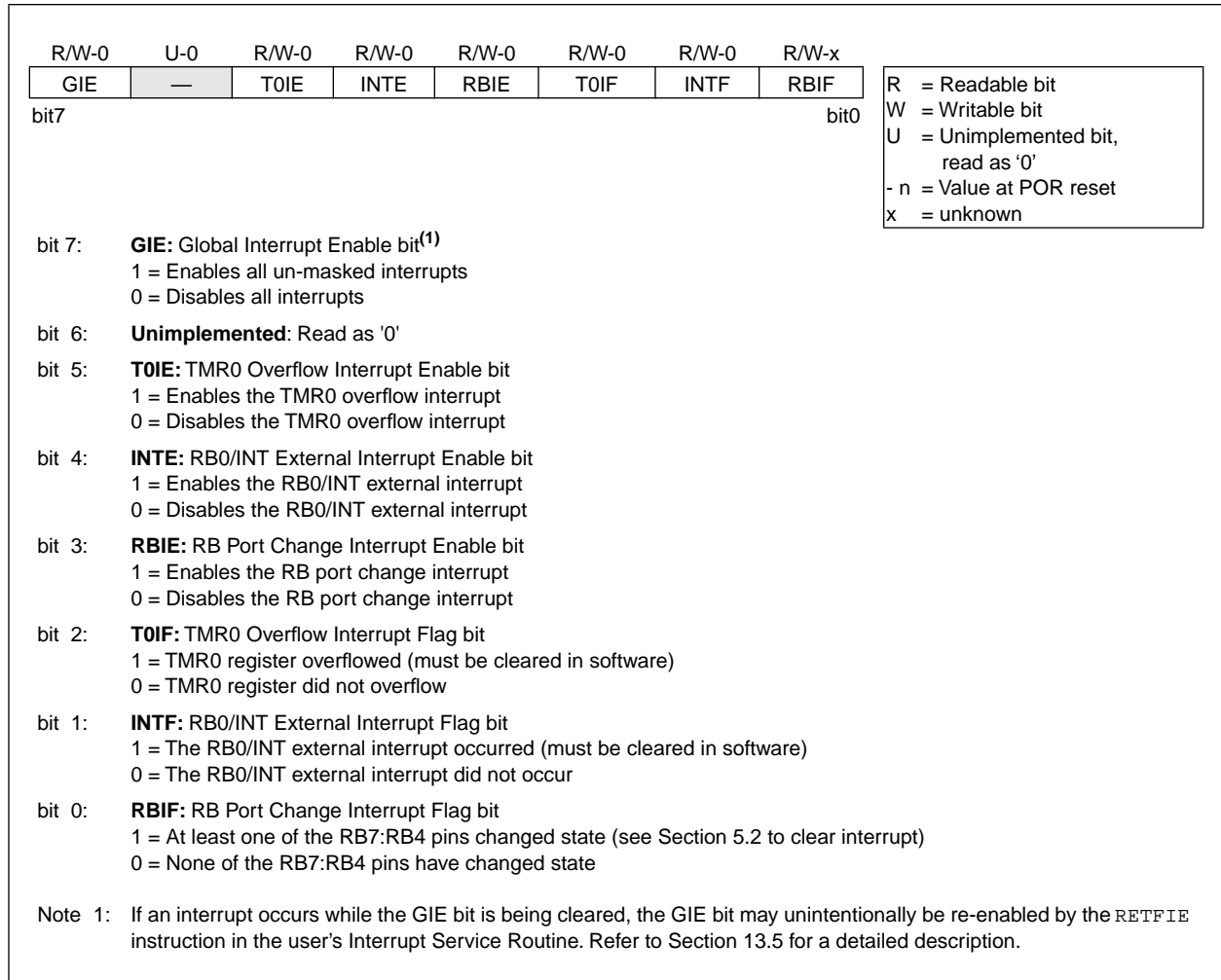
FIGURE 4-9: INTCON REGISTER FOR PIC16C61 (ADDRESS 0Bh, 8Bh)
