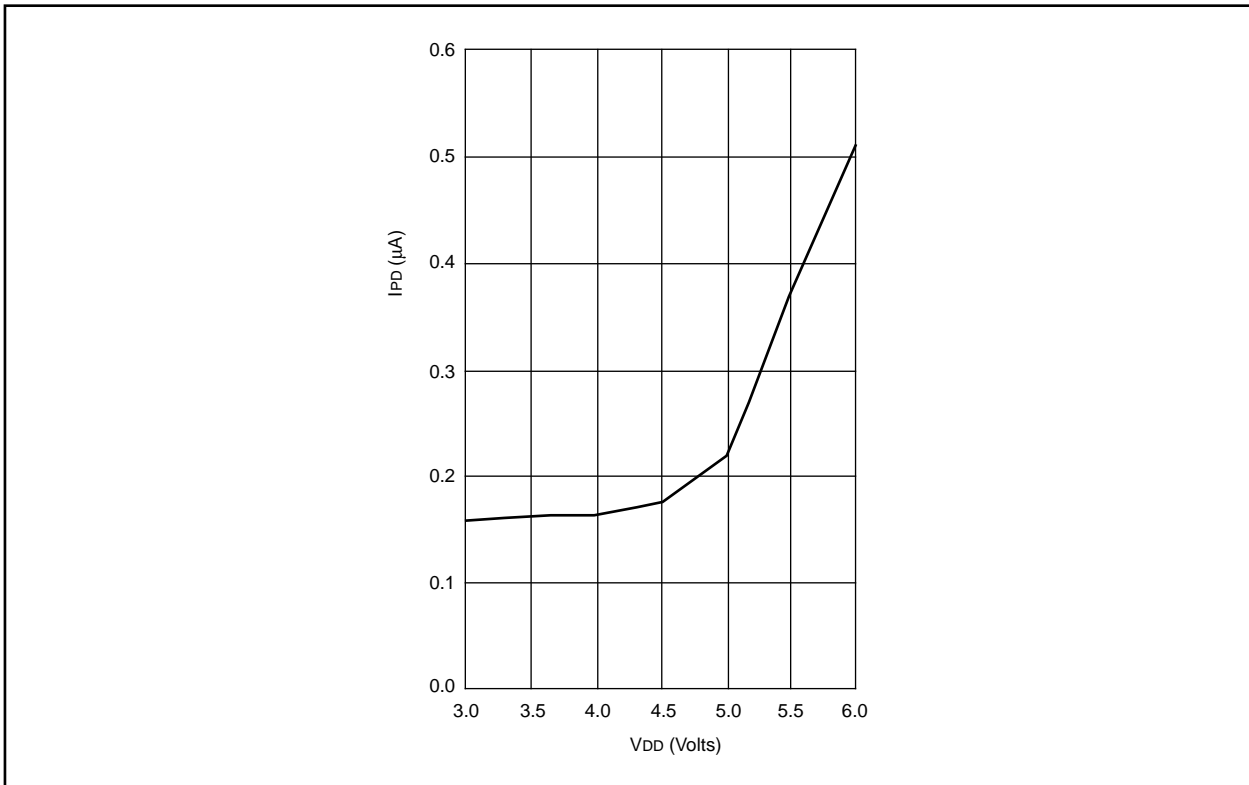
FIGURE 17-5: TYPICAL I_{PD} vs. V_{DD} WATCHDOG TIMER DISABLED 25^\circ\text{C}
